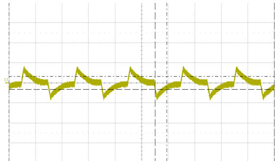
Fig. 12: Output voltage response to load current step-change (10 A – 15 A – 10 A) at V_{in} = 48\ \text{V} . Current slew rate: 0.1\ \text{A}/\mu\text{s} . C_o = 4700\ \mu\text{F} E-cap + 1\ \mu\text{F} ceramic + 10\ \mu\text{F} tantalum. Time scale: 500 \mu\text{s}/\text{div} .
