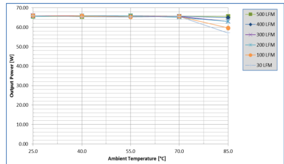
Fig. 6: Power derating vs. ambient air temperature and airflow rates for UIS48T20033 converter with baseplate equipped with .45" finned heatsink mounted vertically with air flowing from pin 3 to pin 1, MOSFET temperature \leq 125^{\circ}\text{C} , V_{in}=48\text{V}
