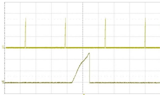
Fig. 17: Load current (top trace, 20 \text{ A}/\text{div} ., 200 \text{ ms}/\text{div} .) into a 10 \text{ m}\Omega short circuit during restart, at V_{in} = 48 \text{ V} . Bottom trace ( 20 \text{ A}/\text{div} ., 10 \text{ ms}/\text{div} .) is an expansion of the on-time portion of the top trace.
