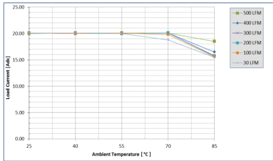
Fig. 1: Available load current vs. ambient air temperature and airflow rates for UIS48T20033 converter w/o baseplate mounted vertically with air flowing from pin 3 to pin 1, MOSFET temperature \leq 125^{\circ}\text{C} , V_{in}=48\text{V}
