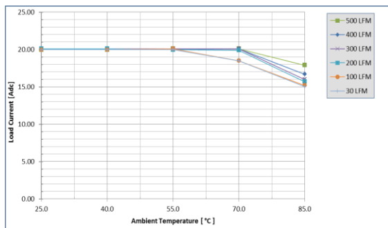
Fig. 3: Available load current vs. ambient air temperature and airflow rates for UIS48T20033 converter w/o baseplate mounted vertically with air flowing from pin 3 to pin 1, MOSFET temperature \leq 125^{\circ}\text{C} , V_{in}=24\text{V}
