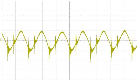
Fig. 13: Output voltage ripple (20 mV/div.) at full rated load current into a resistive load with C_o = 10 \mu\text{F} tantalum + 1 \mu\text{F} ceramic and V_{in} = 48 \text{ V} . Time scale: 2 \mu\text{s}/\text{div}
