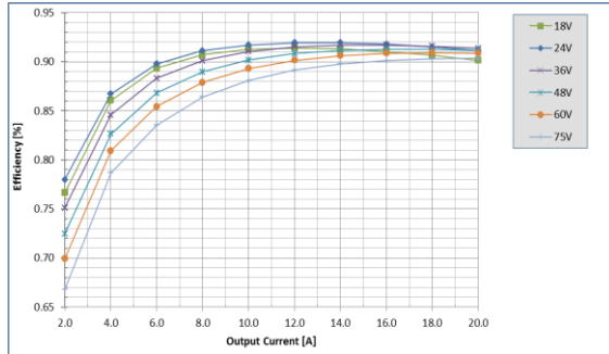
Fig. 7: Efficiency vs. load current and input voltage for UIS48T20033 converter w/o baseplate mounted vertically with air flowing from pin 3 to pin 1 at a rate of 300 LFM (1.5 m/s) and T_a = 25^\circ\text{C} .
