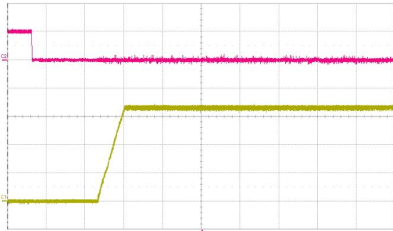
Fig. 9: Turn-on transient at full rated load current (resistive) with C_{out} = 10\ \mu\text{F} tantalum + 1\ \mu\text{F} ceramic at V_{in} = 48\ \text{V} , triggered via ON/OFF pin. Top trace: ON/OFF signal (5 V/div.). Bottom trace: output voltage (1 V/div.). Time scale: 50 ms/div.
