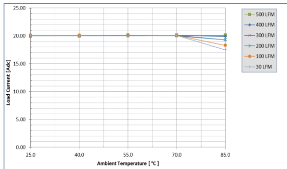
Fig. 5: Available load current vs. ambient air temperature and airflow rates for UIS48T20033 converter with baseplate equipped with .45" finned heatsink mounted vertically with air flowing from pin 3 to pin 1, MOSFET temperature \leq 125^{\circ}\text{C} , V_{in}=48\text{V}
