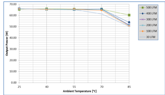
Fig. 2: Power derating vs. ambient air temperature and airflow rates for UIS48T20033 converter w/o baseplate mounted vertically with air flowing from pin 3 to pin 1, MOSFET temperature \leq 125^{\circ}\text{C} , V_{in}=48\text{V}
