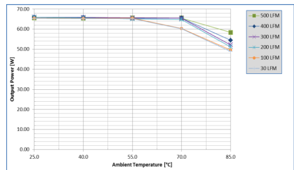
Fig. 4: Power derating vs. ambient air temperature and airflow rates for UIS48T20033 converter w/o baseplate mounted vertically with air flowing from pin 3 to pin 1, MOSFET temperature \leq 125^{\circ}\text{C} , V_{in}=24\text{V}
