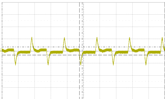
Fig. 11: Output voltage response to load current step-change (10 A – 15 A – 10 A) at V_{in} = 48\ \text{V} . Current slew rate: 0.1\ \text{A}/\mu\text{s} . C_o = 470\ \mu\text{F} E-cap + 1\ \mu\text{F} ceramic + 10\ \mu\text{F} tantalum. Time scale: 500 \mu\text{s}/\text{div} .
