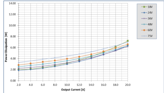
Fig. 8: Power dissipation vs. load current and input voltage for UIS48T20033 converter w/o baseplate mounted vertically with air flowing from pin 3 to pin 1 at a rate of 300 LFM (1.5 m/s) and T_a = 25^\circ\text{C} .
