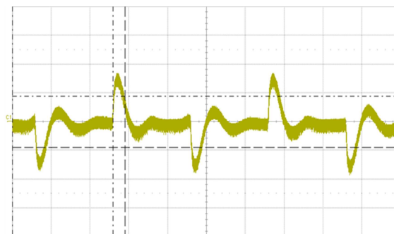
Fig. 12: Output voltage response to load current step-change (3A – 4.5A – 3A) at V_{in} = 48 \text{ V} . Current slew rate: 0.1 \text{ A}/\mu\text{s} . C_o = 270 \mu\text{F} E-cap + 1 \mu\text{F} ceramic + 10 \mu\text{F} tantalum. Time scale: 500 \mu\text{s}/\text{div} .
