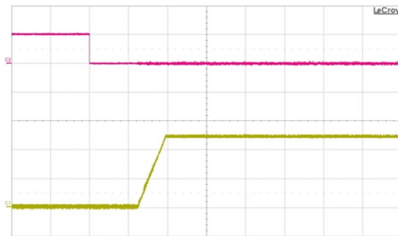
Fig. 9: Turn-on transient at full rated load current (resistive) with C_{out} = 10 \mu\text{F} tantalum + 1 \mu\text{F} ceramic at V_{in} = 48 \text{ V} , triggered via ON/OFF pin. Top trace: ON/OFF signal (5 V/div.). Bottom trace: output voltage (5 V/div.). Time scale: 50 ms/div
