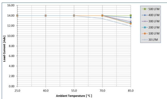
Fig. 3: Available load current vs. ambient air temperature and airflow rates for UIS48T14050 converter w/o baseplate mounted vertically with air flowing from pin 3 to pin 1, MOSFET temperature \leq 125^{\circ}\text{C} , V_{in}=24\text{V}
