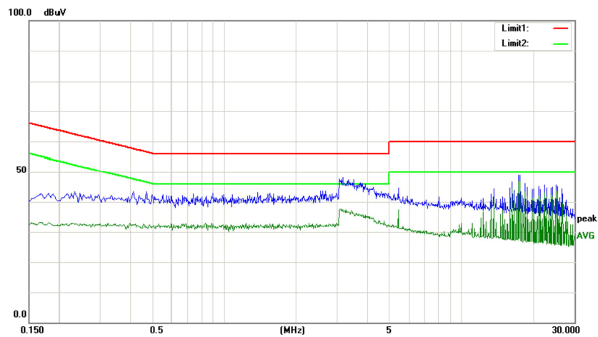
Fig. 19: Vin+ Peak Detector EMI waveform
