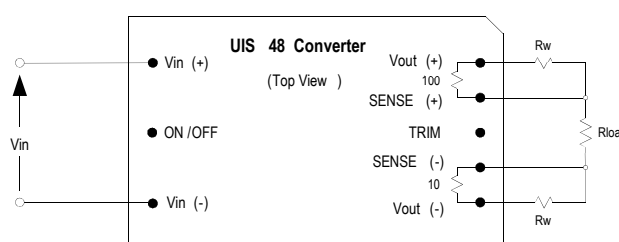
Fig. B: Remote sense circuit configuration.
