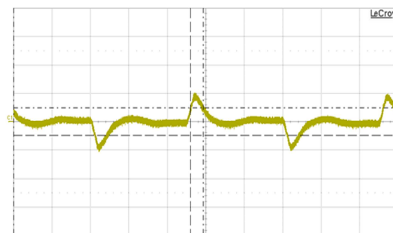
Fig. 11: Output voltage response to load current step-change (7A - 10.5 A - 7 A) at V_{in} = 48\text{ V} . Current slew rate: 0.1 A/ \mu\text{s} . C_o = 470\mu\text{F} E-cap + 1 \mu\text{F} ceramic + 10 \mu\text{F} tantalum. Time scale: 100 \mu\text{s} /div.
