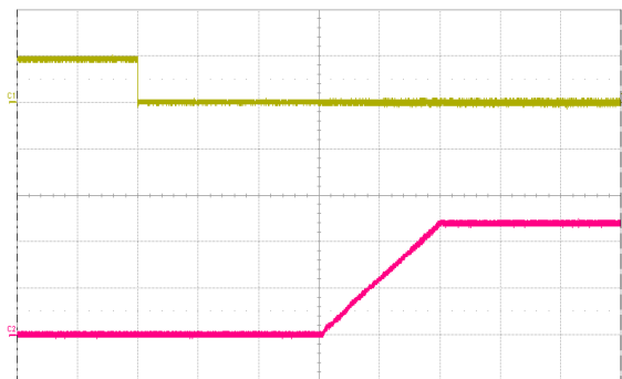
Fig. 10: Turn-on transient at full rated load current (resistive) plus 4,700 \mu\text{F} at V_{in} = 48 \text{ V} , triggered via ON/OFF pin. Top trace: ON/OFF signal (5 V/div.). Bottom trace: output voltage (5 V/div.). Time scale: 20 ms/div.
