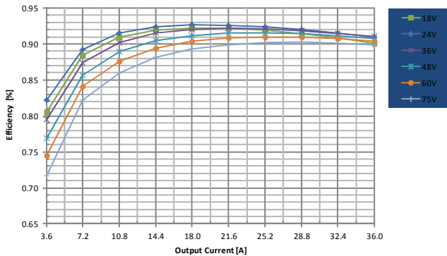
Fig. 7: Efficiency vs. load current and input voltage for UIE48T36033 converter w/o baseplate mounted vertically with air flowing from pin 3 to pin 1 at a rate of 300 LFM (1.5 m/s) and T_a = 25^\circ\text{C} .
