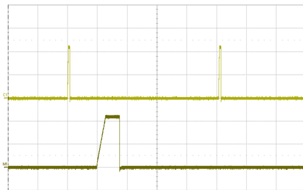
Fig. 17: Load current (top trace, 20 \text{ A}/\text{div} , 100 \text{ ms}/\text{div} .) into a 10 \text{ m}\Omega short circuit during restart, at V_{in} = 48 \text{ V} . Bottom trace ( 20 \text{ A}/\text{div} ., 10 \text{ ms}/\text{div} .) is an expansion of the on-time portion of the top trace
