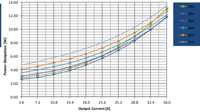
Fig. 8: Power dissipation vs. load current and input voltage for UIE48T36033 converter w/o baseplate mounted vertically with air flowing from pin 3 to pin 1 at a rate of 300 LFM (1.5 m/s) and T_a = 25^\circ\text{C} .
