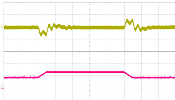
Fig. 11: Output voltage response to load current step change (18A – 27A – 18A) at V_{in} = 48 \text{ V} . Top trace: output voltage (200 mV/div.). Bottom trace: load current (20 A/div.). Current slew rate: 0.1 \text{ A}/\mu\text{s} . C_o = 1 \mu\text{F} ceramic + 10 \mu\text{F} tantalum. Time scale: 200 \mu\text{s}/\text{div} .
