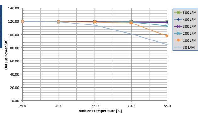
Fig. 6: Power derating vs. ambient air temperature and airflow rates for UIE48T36033 converter with baseplate equipped with .45" finned heatsink mounted vertically with air flowing from pin 3 to pin 1, MOSFET temperature \leq 125^{\circ}\text{C} , V_{in}=48\text{V}
