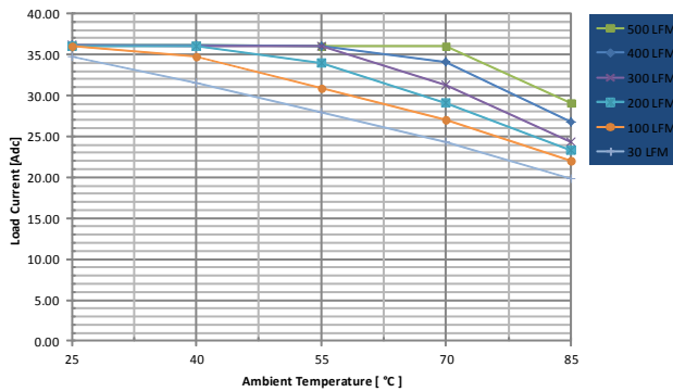
Fig. 3: Available load current vs. ambient air temperature and airflow rates for UIE48T36033 converter w/o baseplate mounted vertically with air flowing from pin 3 to pin 1, MOSFET temperature \leq 125^{\circ}\text{C} , V_{in}=24\text{V}
