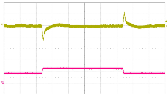
Fig. 12: Output voltage response to load current step change (18A – 27A – 18A) at V_{in} = 48 \text{ V} . Top trace: output voltage (200 mV/div.). Bottom trace: load current (20 A/div.). Current slew rate: 1 \text{ A}/\mu\text{s} . C_o = 1 \mu\text{F} ceramic + 10,000 \mu\text{F} + 10 \mu\text{F} tantalum. Time scale: 200 \mu\text{s}/\text{div} .
