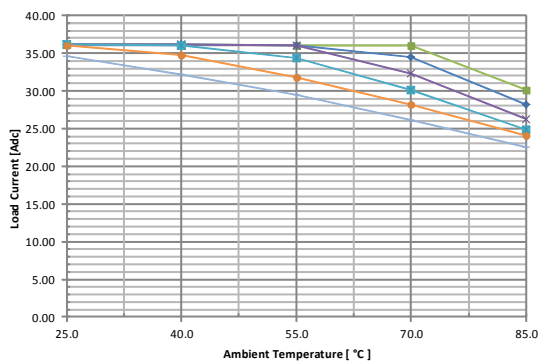
Fig. 3: Available load current vs. ambient air temperature and airflow rates for UIE48T36033 converter w/o baseplate mounted vertically with air flowing from pin 3 to pin 1, MOSFET temperature \leq 125^{\circ}\text{C} , V_{in}=24\text{V}
