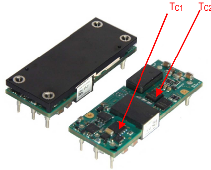
Fig. G: Locations of the thermocouples for thermal testing.
