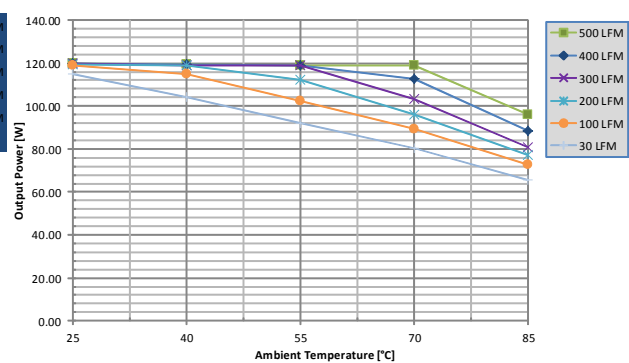
Fig. 4: Power derating vs. ambient air temperature and airflow rates for UIE48T36033 converter w/o baseplate mounted vertically with air flowing from pin 3 to pin 1, MOSFET temperature \leq 125^{\circ}\text{C} , V_{in}=24\text{V}
