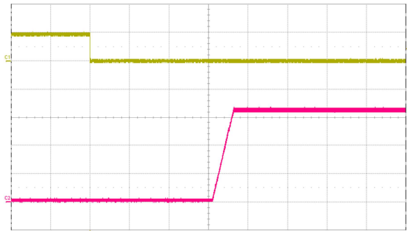
Fig. 10: Turn-on transient at full rated load current (resistive) plus 10,000 \mu\text{F} at V_{in} = 48 \text{ V} , triggered via ON/OFF pin. Top trace: ON/OFF signal (5 V/div.). Bottom trace: output voltage (1 V/div.). Time scale: 20 ms/div.
