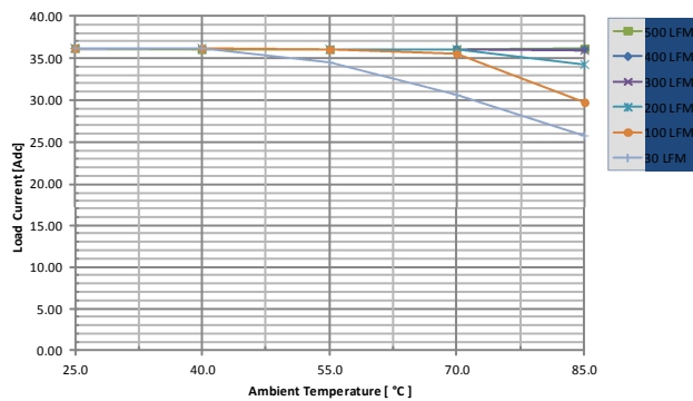
Fig. 5: Available load current vs. ambient air temperature and airflow rates for UIE48T36033 converter with baseplate equipped with .45" finned heatsink mounted vertically with air flowing from pin 3 to pin 1, MOSFET temperature \leq 125^{\circ}\text{C} , V_{in}=48\text{V}
