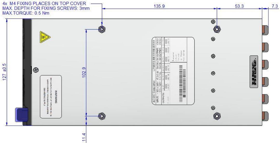
Figure 9 - Top View
